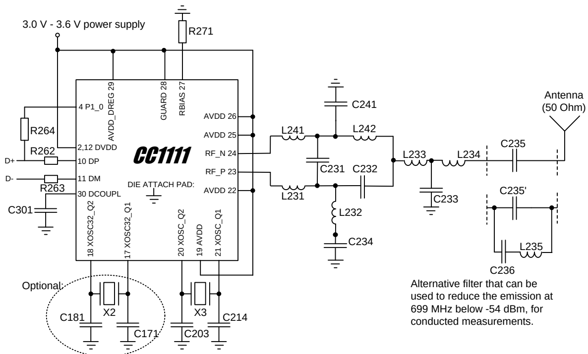
Figure 12: Application Circuit for CC1111F 868/915 MHz with Fundamental Crystal (excluding supply decoupling capacitors)
