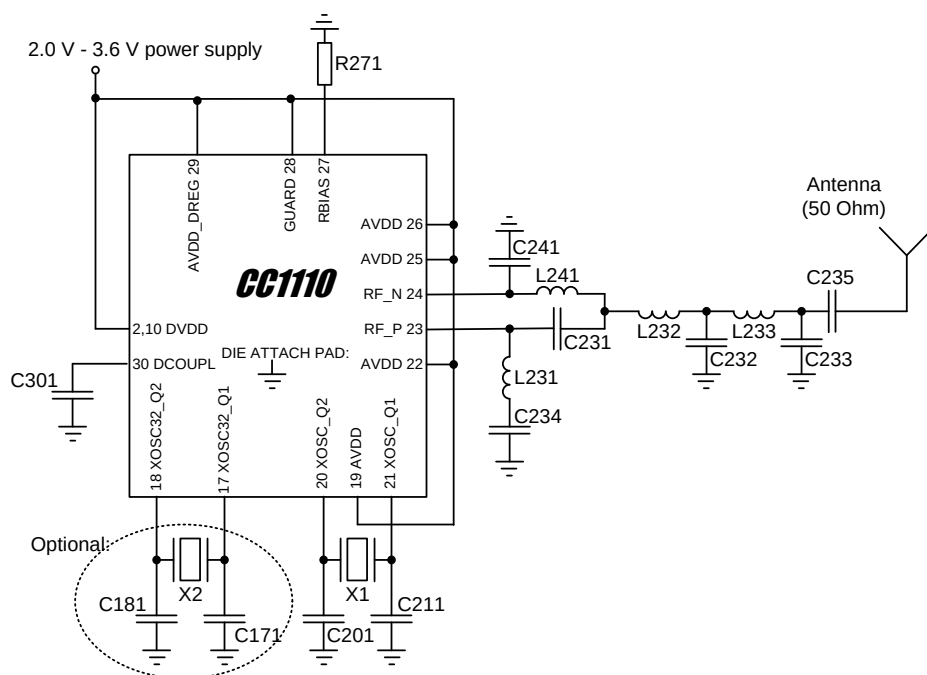
Figure 10: Application Circuit for CC1100 315/433 MHz (excluding supply decoupling capacitors)
